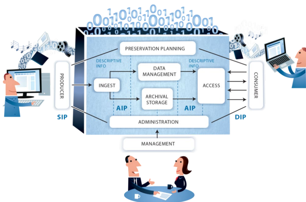
Figure 1: OAIS reference model drawn by digitalbevaring.dk
